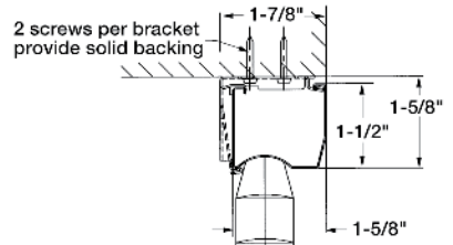
Inside Mounted Detail
