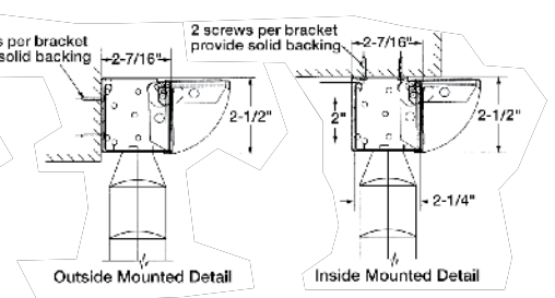
Note: Bracket detail for RIV2
