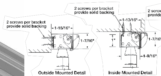
Note: Bracket detail for RIV1, RIV1P, RIV1C, RIV1-S
